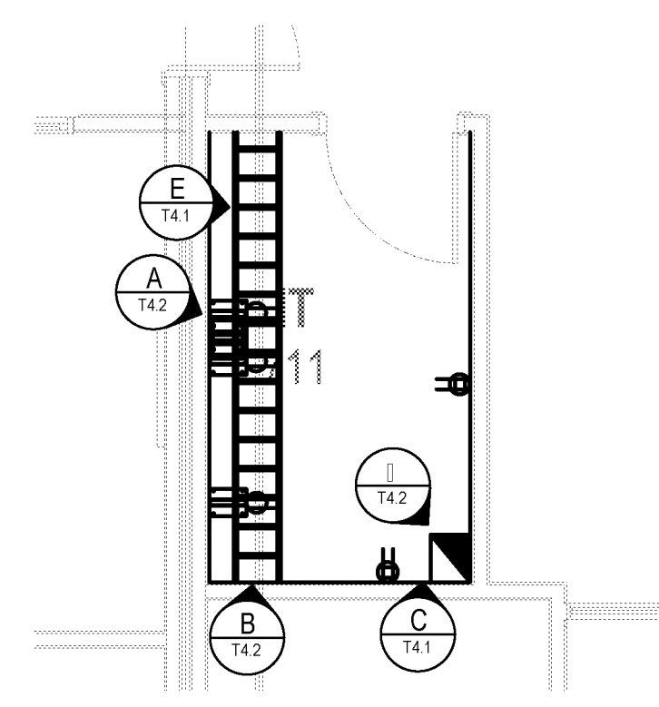
2 ENLARGED IT ROOM #711 1/4" = 10'
