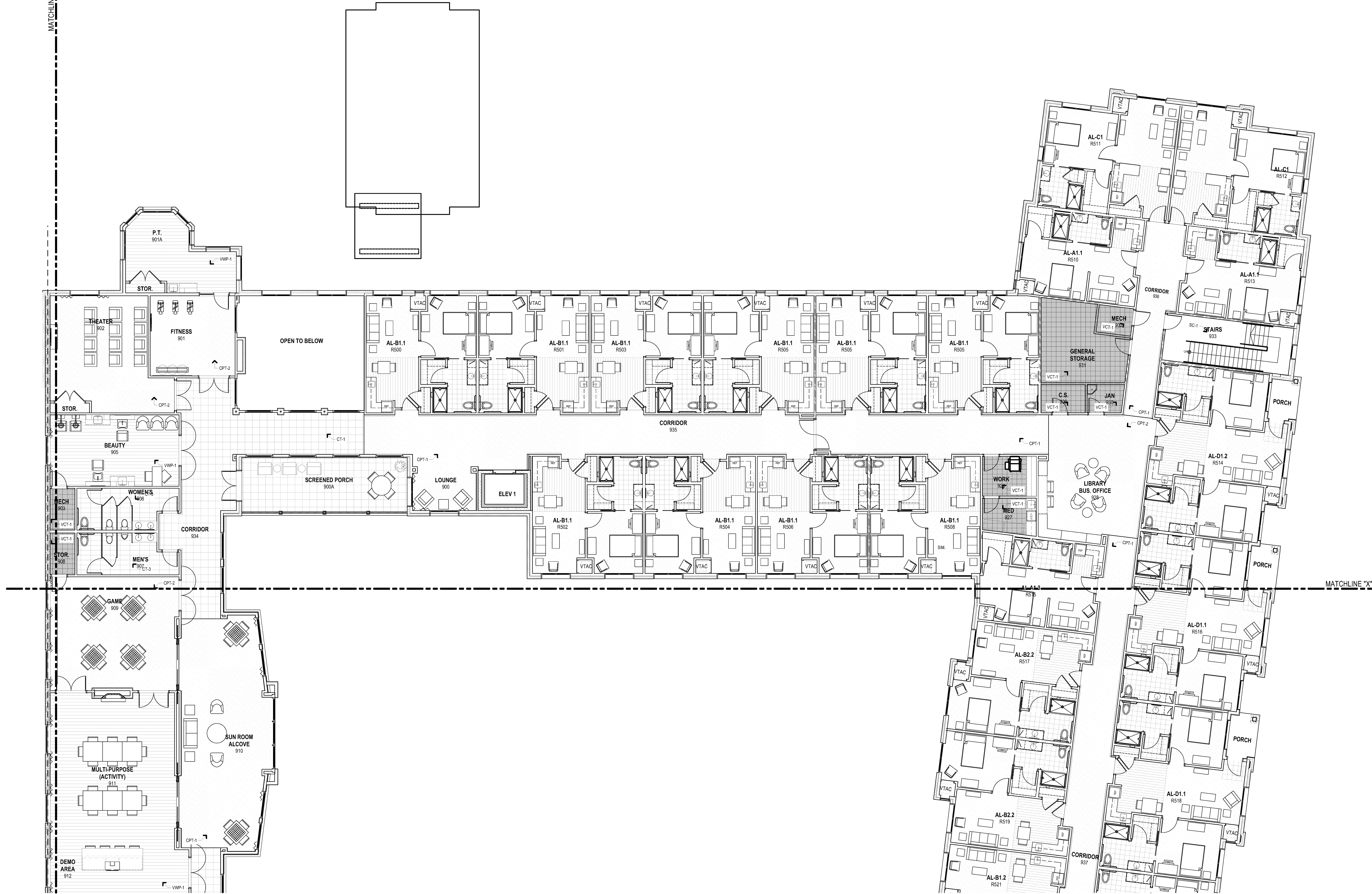
A1 ENLARGED SECOND FLOOR FINISH PLAN (NE) SCALE: 1/8" = 1'-0"
