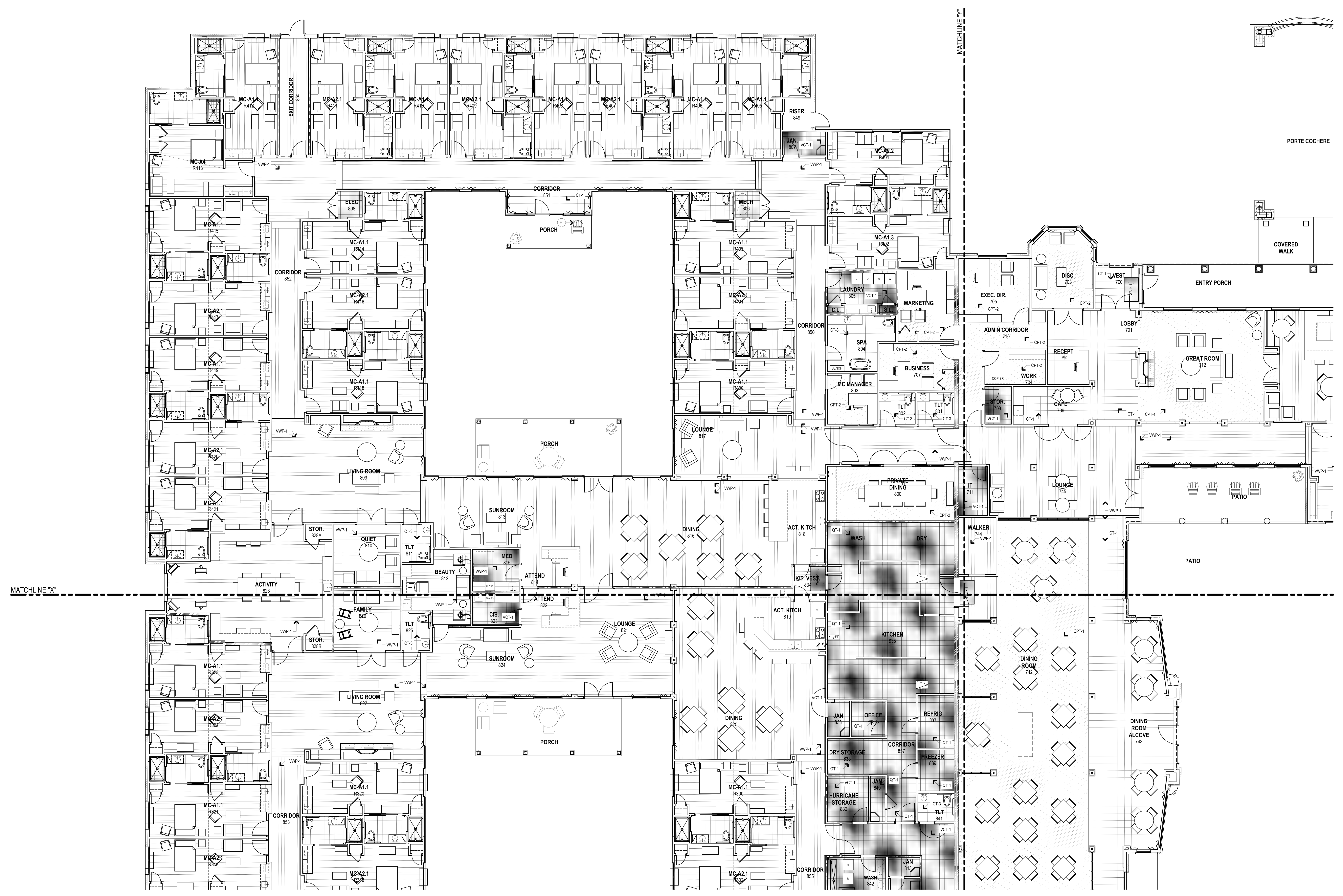
A1 ENLARGED FIRST FLOOR FINISH PLAN (NW) SCALE: 1/8" = 1'-0"
