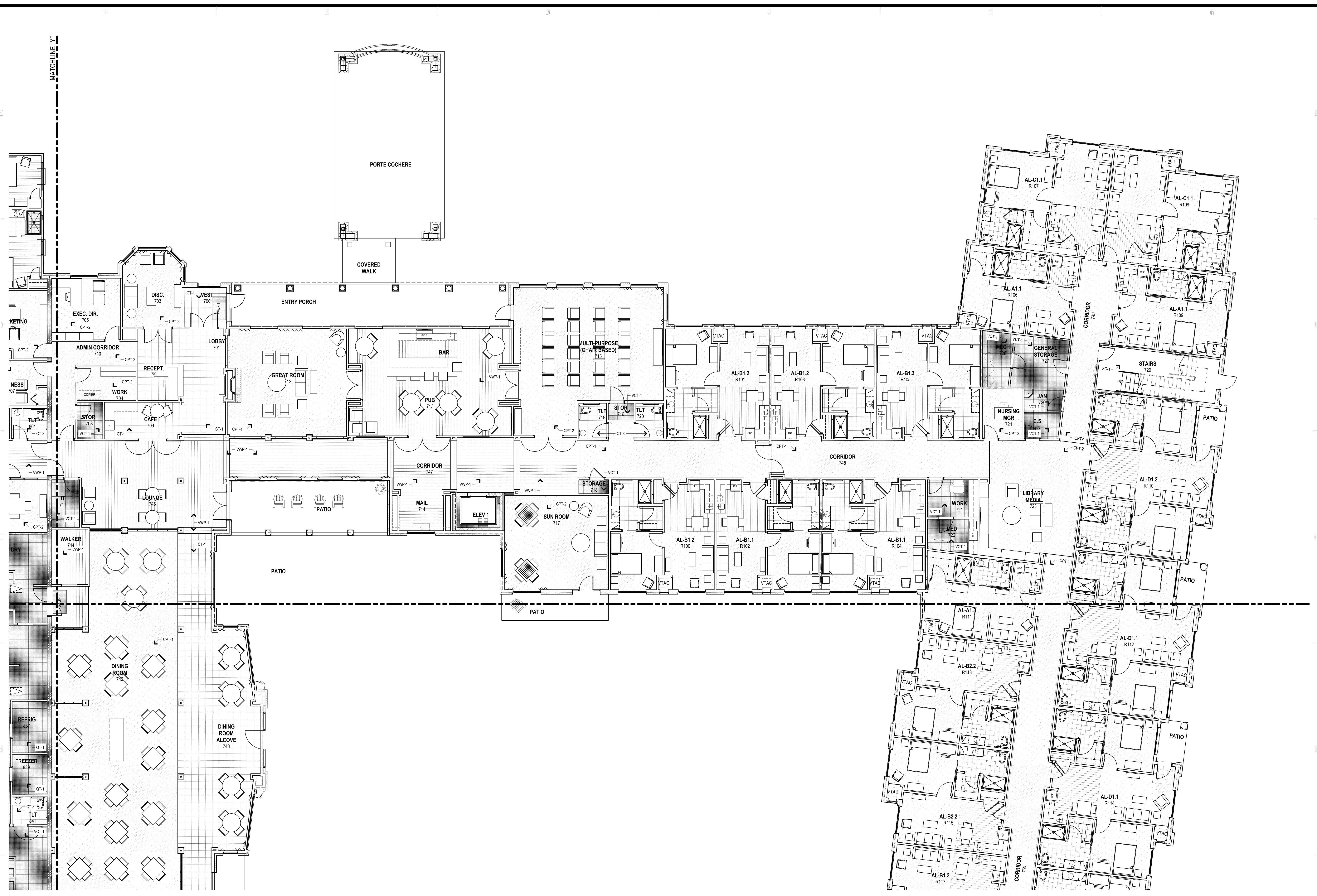
A1 ENLARGED FIRST FLOOR FINISH PLAN (NE) SCALE: 1/8" = 1'-0"
