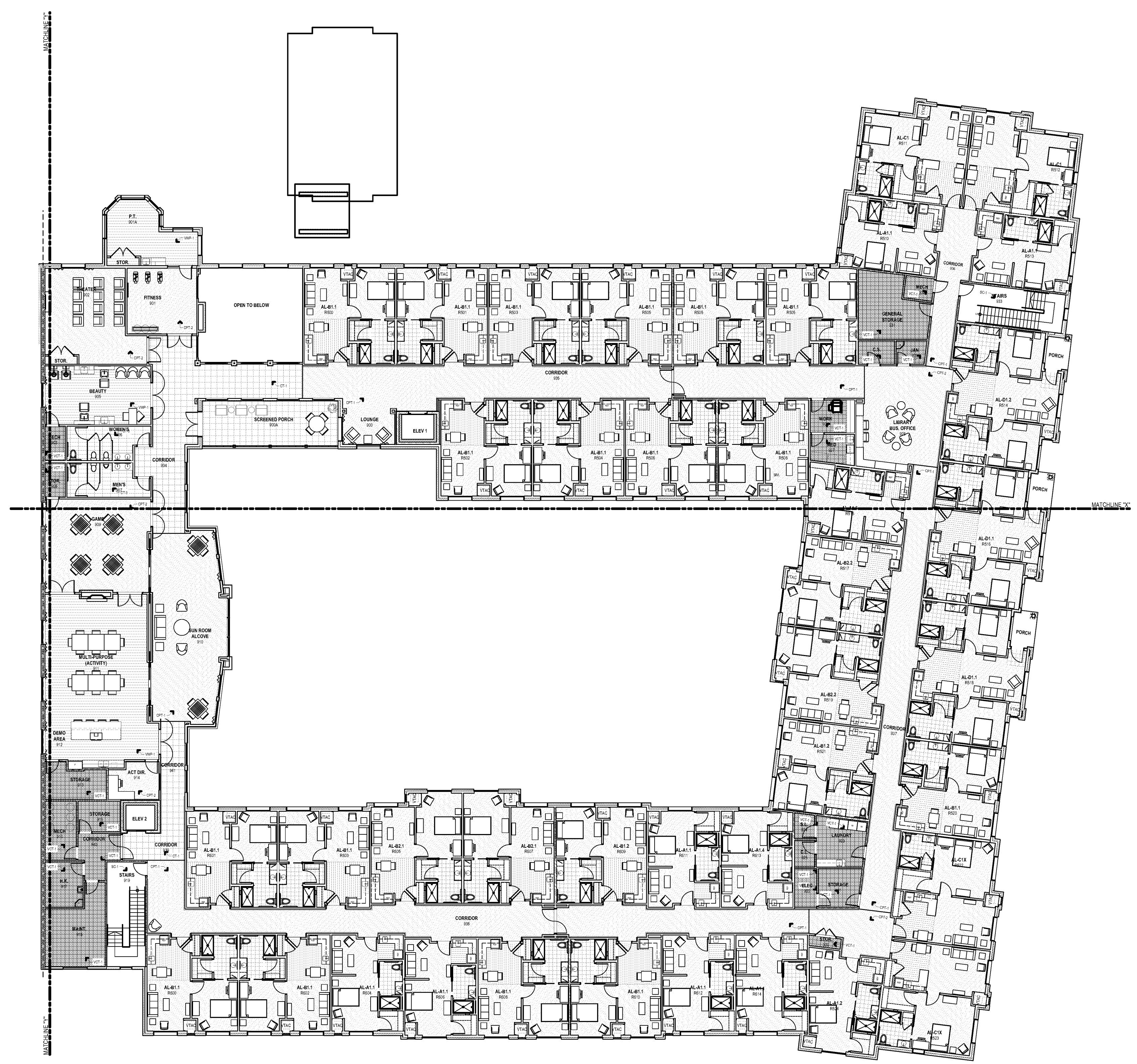
B3 OVERALL SECOND FLOOR FINISH PLAN SCALE: 1/16" = 1'-0"
