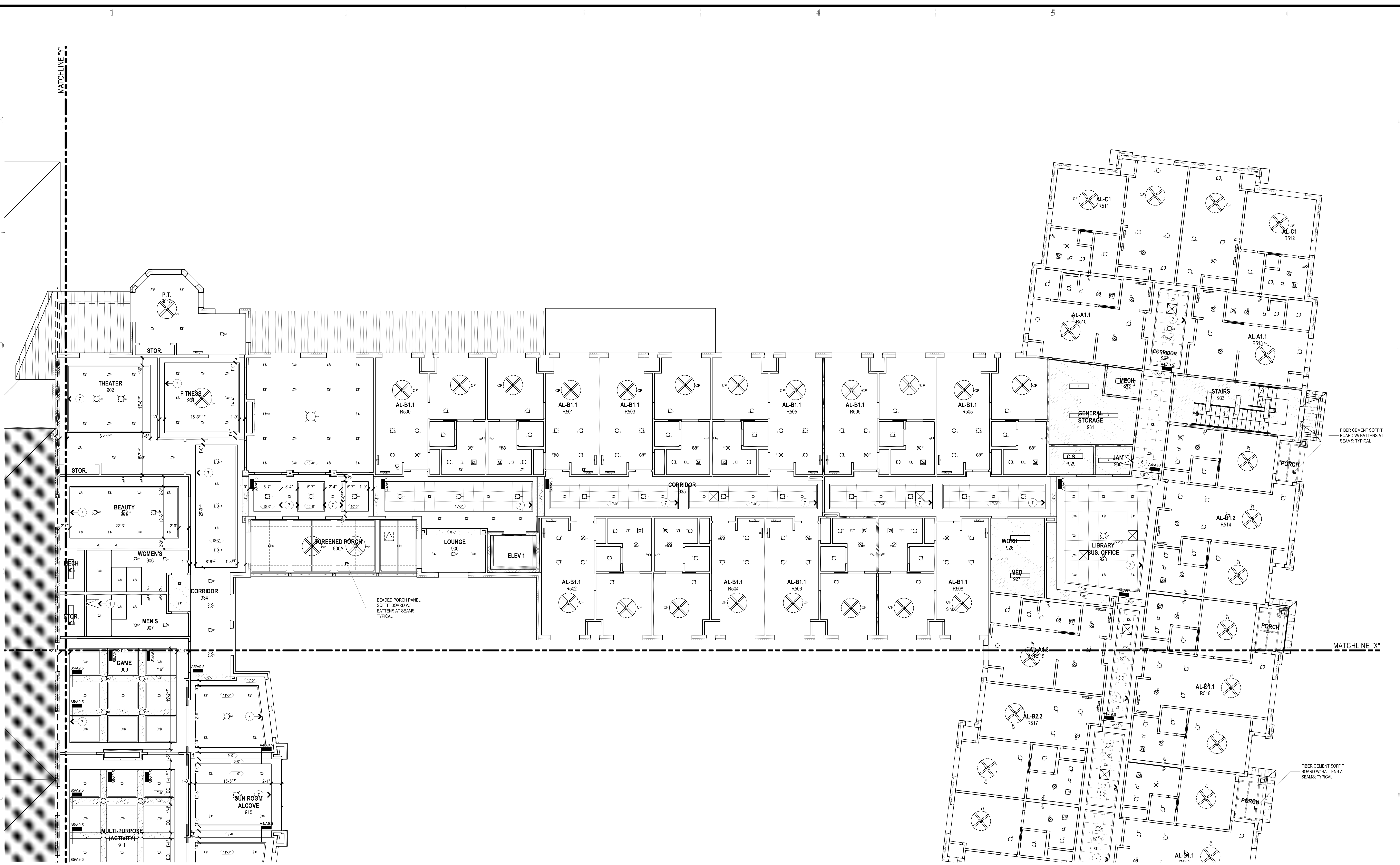
B1 SECOND FLOOR REFLECTED CEILING PLAN SCALE: 1/8" = 1'-0"
