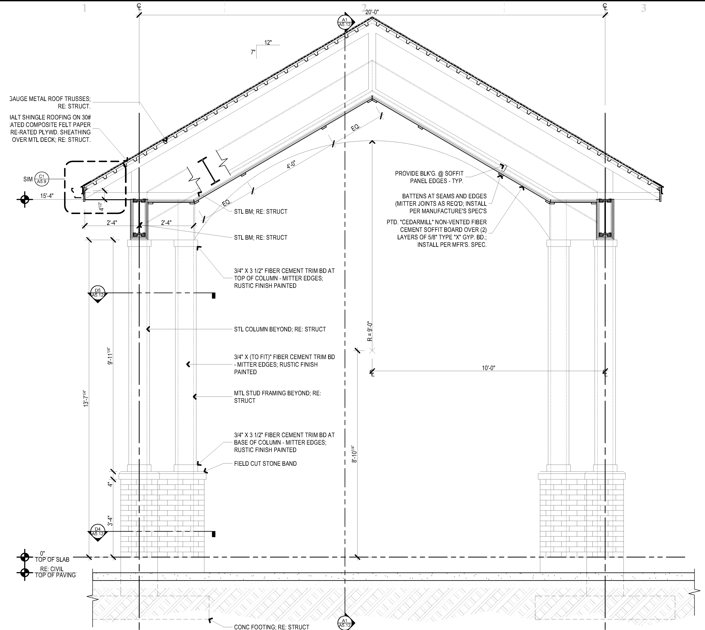
C1 WS-A5.13 SECTION 02 @ PORTE COCHERE SCALE: 1/2" = 1'-0"
