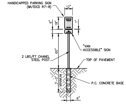
18 HANDICAPPED PARKING SIGN (VAN ACCESSIBLE) SCALE: N.T.S.
