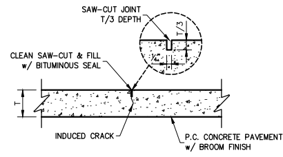
6 TYPICAL CONTRACTION JOINT "C" - ALT 2 P.C. CONCRETE PAVEMENT SCALE: N.T.S.
