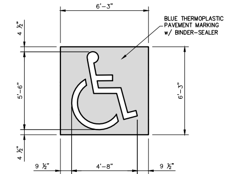
17 ADA STANDARD PARKING PAVEMENT SYMBOL THERMOPLASTIC BLUE SYMBOL SCALE: N.T.S.
