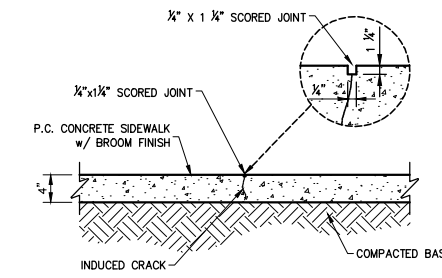
4 4" P.C. CONCRETE SIDEWALK SECTION w/ TYPICAL DUMMY (CONTROL JOINT) SCALE: N.T.S.
