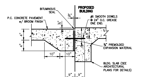
20 CONCRETE SIDEWALK SECTION TO BUILDING SLAB CONNECTION ALL AREAS SCALE: N.T.S.
