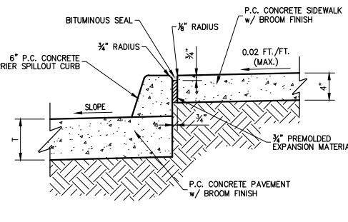
12 TYPICAL SECTION 4" SIDEWALK / SPILLOVER CURB 6" BARRIER SPILLOVER CURB SCALE: N.T.S.
