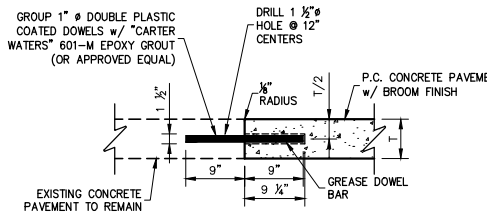
10 TYPICAL TIE TO EXISTING CONCRETE PAVEMENT - ALT 1 P.C. CONCRETE PAVEMENT SCALE: N.T.S.
