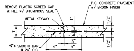
5 TYPICAL CONTRACTION JOINT "C" - ALT 1 P.C. CONCRETE PAVEMENT SCALE: N.T.S.
