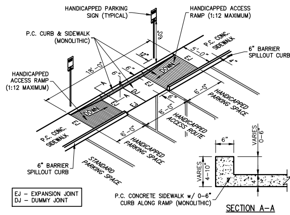
16 HANDICAP RAMP DETAIL 8-FT. ACCESS ROUTE WITH 5-FT. SIDEWALK SCALE: N.T.S.
