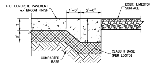
14 LIMESTONE AND CONCRETE PAVEMENT SECTION/CONNECTION PARKING AREA SCALE: N.T.S.
