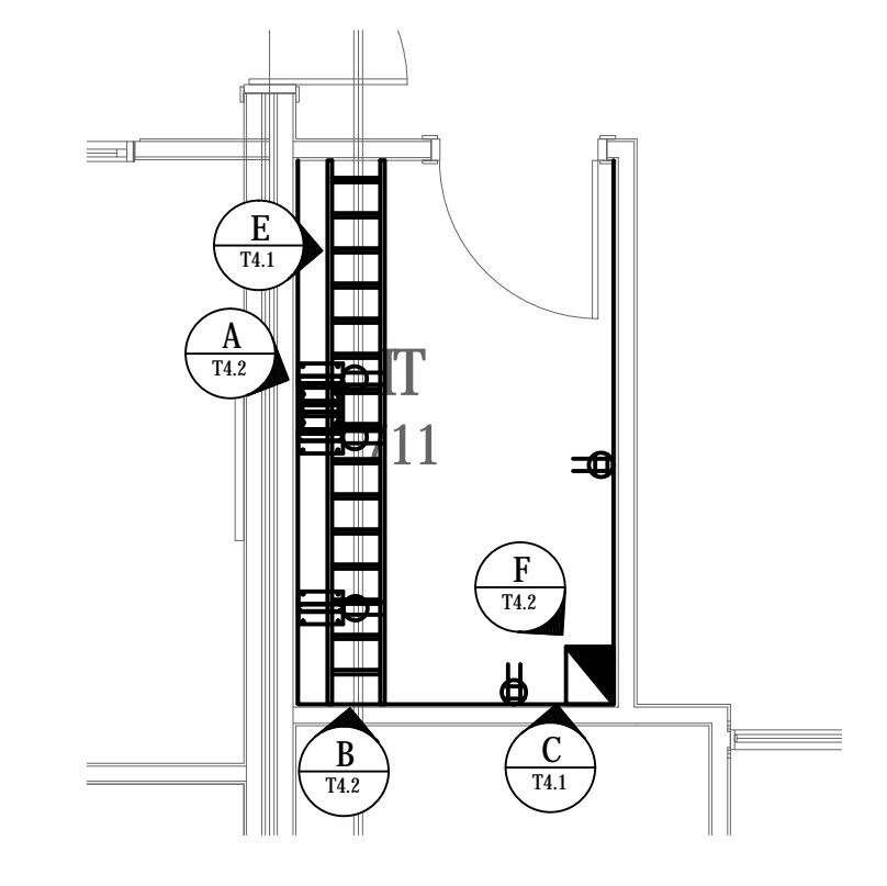
2 ENLARGED IT ROOM #711 1/4" = 1'-0" 0 2 5 8 FT.
